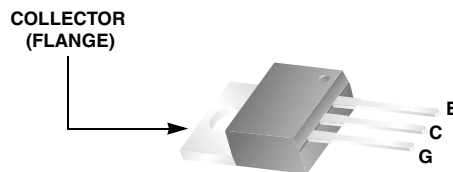
JEDEC TO-220AB (ALTERNATE VERSION)
